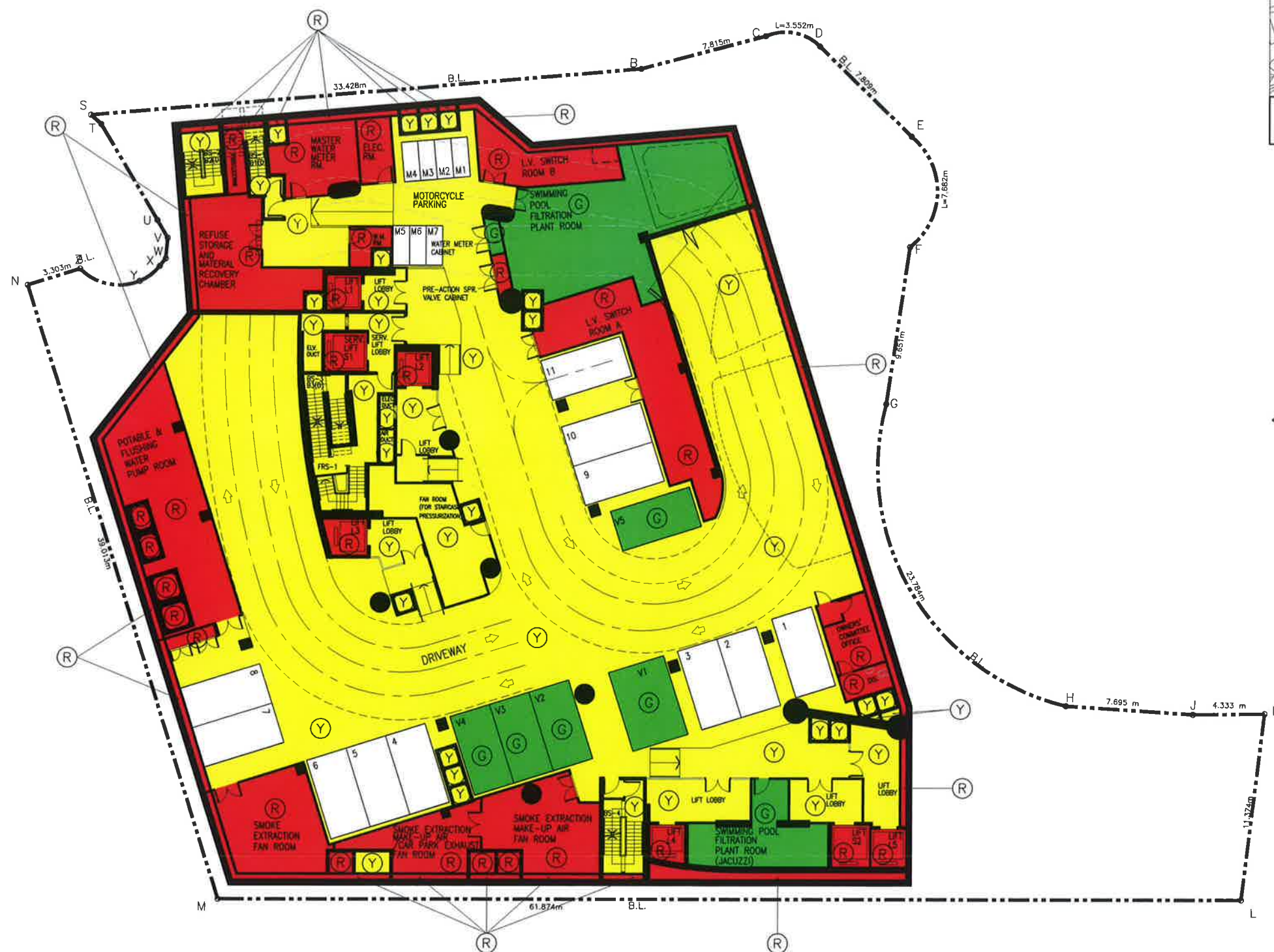
BASEMENT 1 FLOOR PLAN
